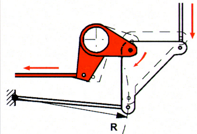
Collective pitch lever up
