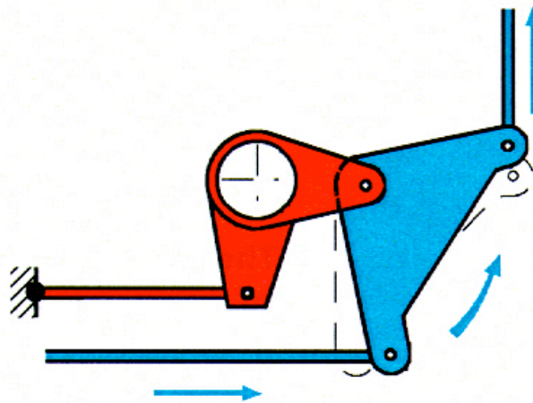
Cyclic stick forward
